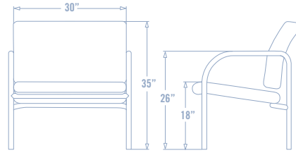
2000 Series Bariatric - Seating Dimensions
