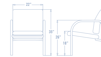
2000 Series - Seating Dimensions
