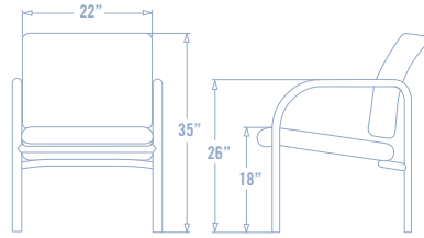
2000 Series - Seating Dimensions
